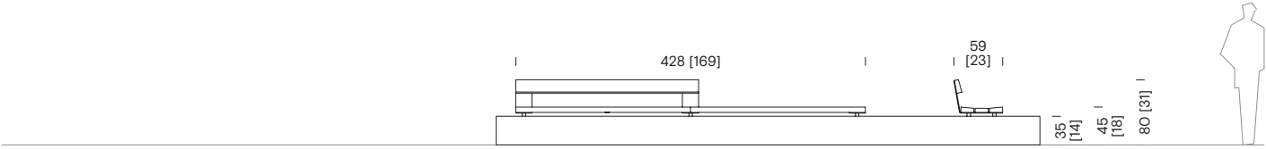
Bench - one section without backrest on a low wall BSB+104
