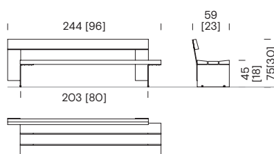
Bench - one section with backrest BCB+114
