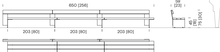
Bench - three sections with three backs BCB+314
