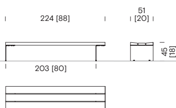
Bench - one section without backrest BCB+104
