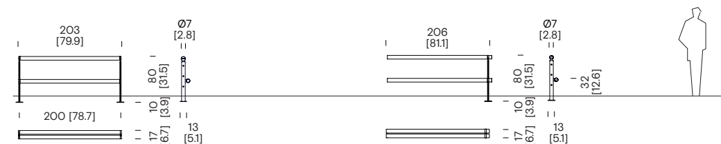
Single-section handrail with beam
