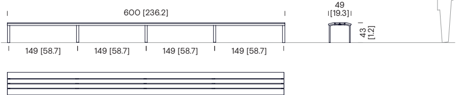
6.00 m Stool NBB51 Aluminium
