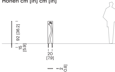
Poller TAP11
